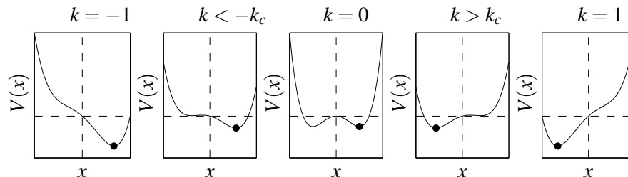
Figure 1. Shape of the potential function V(x) for five values of k . Adapted from Tuller et al. (1994).
