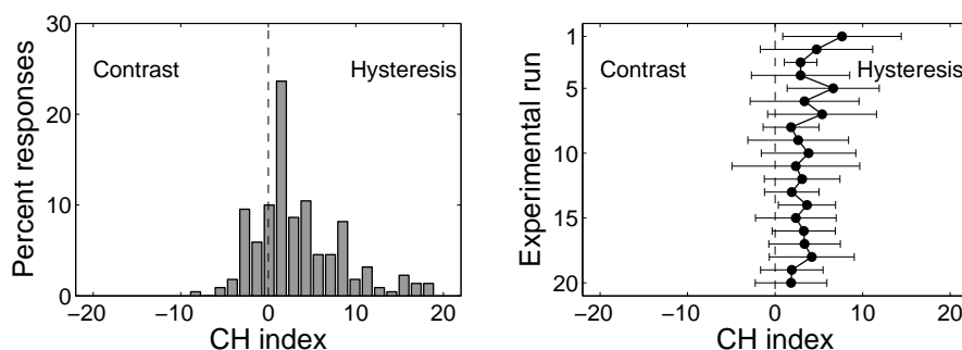
Figure 2. Observed values of the CH index in Nguyen, Lancia and Tuller's (2007a) speech categorization experiment. Left panel: distribution across all the presentations; right panel: mean value and standard deviation for each of the 20 sequential presentations.
